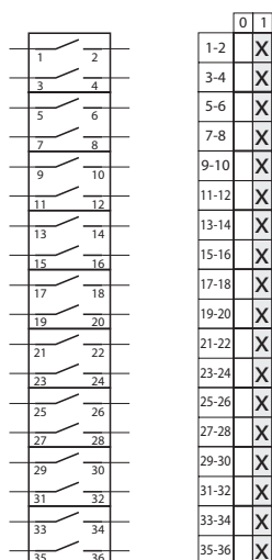
9.821 Disconnector 0-1 (18 - pole)
