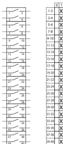
10.821 Disconnector 0-1 (20 - pole)
