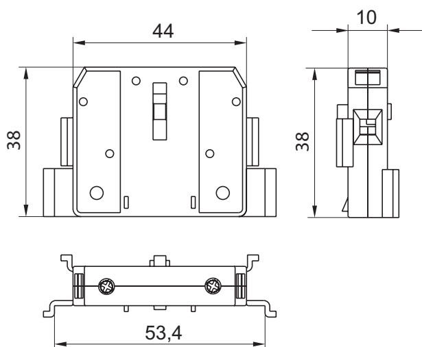
normally open
